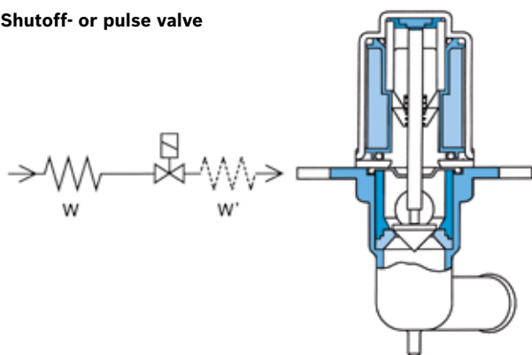
Changeover valve or pulse valve
